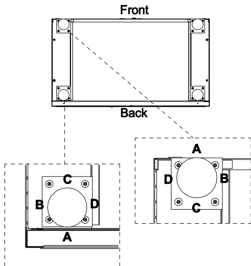
view from under the cabinet
