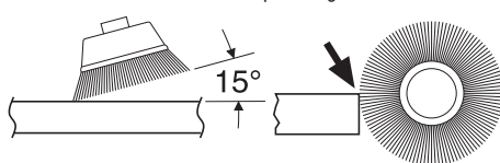
CORRECT: Wire tips doing the work.
