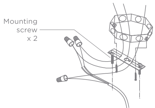
Mounting screw
