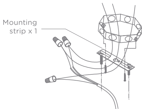
Mounting strip
