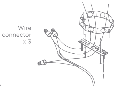
Wire connector
