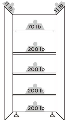
30" Tall Cabinet Max 892 lb (405 kg)
