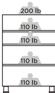
24" 4-drawer Base Cabinet Max 640 lb (290 kg)
