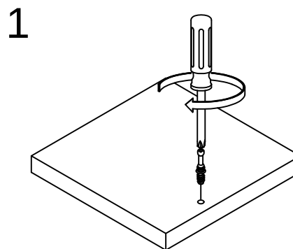
(9) x2 #A12210 1/2" pan head cabeza redondo 1/2" tête ronde 1/2"
