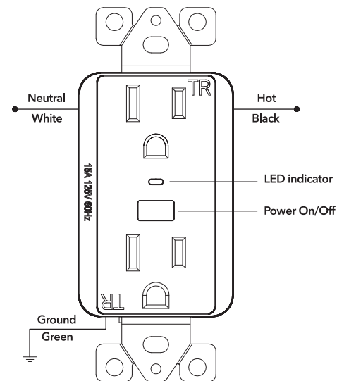
Wiring diagram
