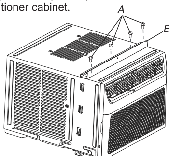
A. 3/8" screws B. Top rail
